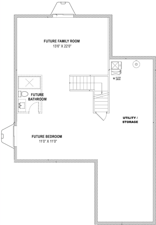
basement
