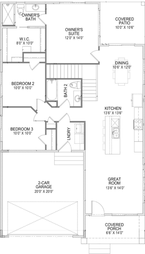
main floor
